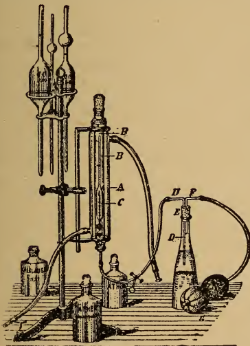
Fig. 59. SOXHLET'S APPARATUS FOR DETERMINING FAT IN MILK.
